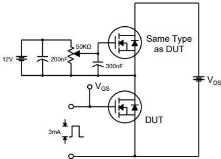
Figure 10. Gate Charge Test Circuit & Waveforms
